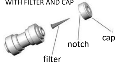
QUICK-CONNECT FITTING WITH FILTER AND CAP
